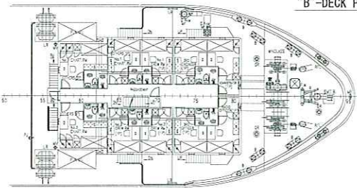
"B"-DECK PLAN
