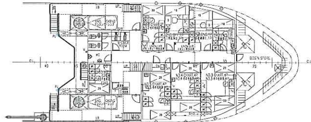
"A"-DECK PLAN
