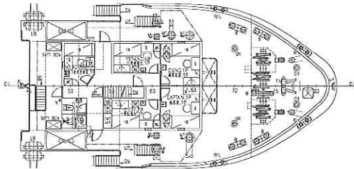
"B"-DECK PLAN
