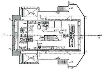
"B"-DECK PLAN
