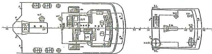
COMPASS DECK
